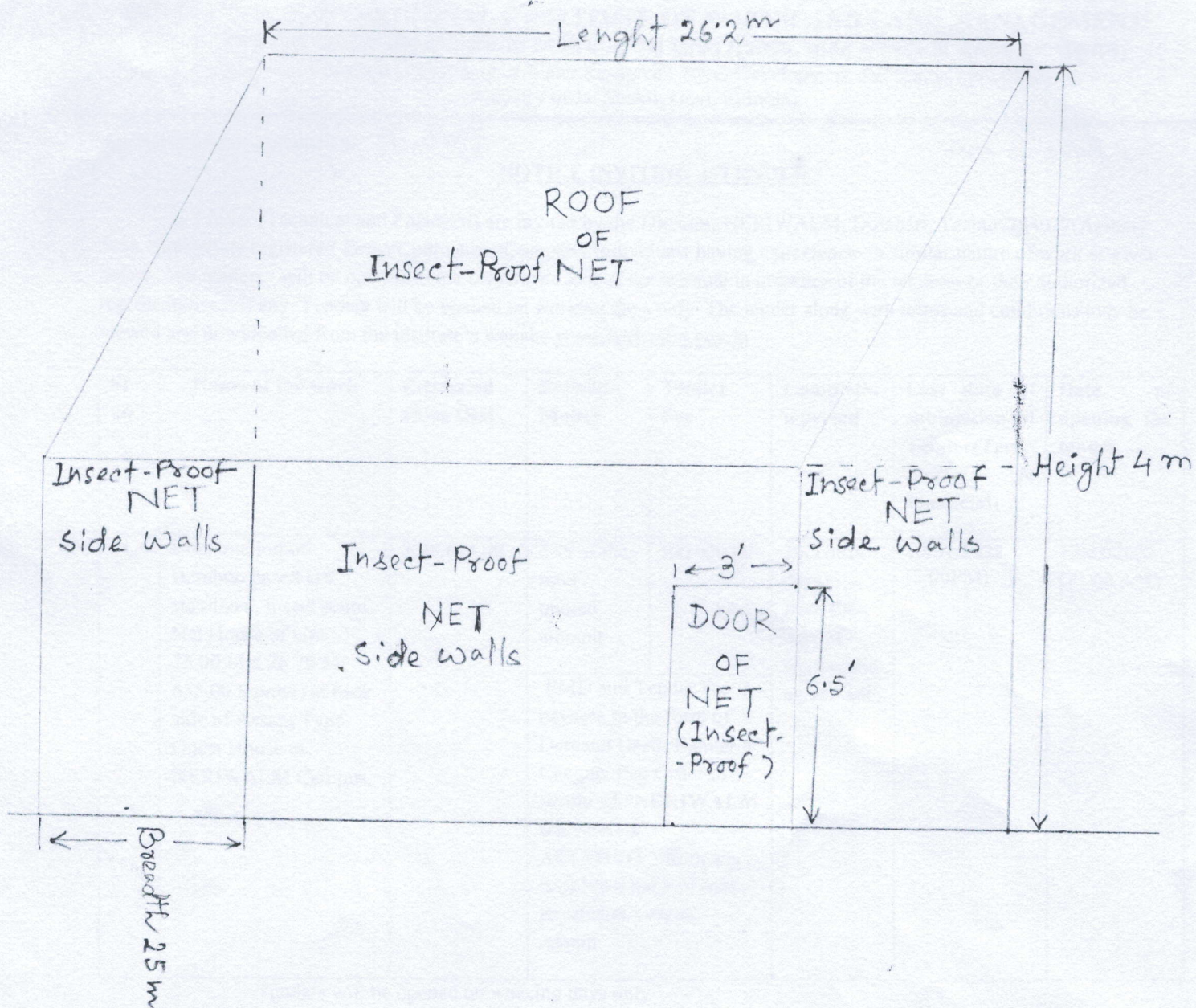
Fig: Sketch of the Proposed Insect Proof Net House
